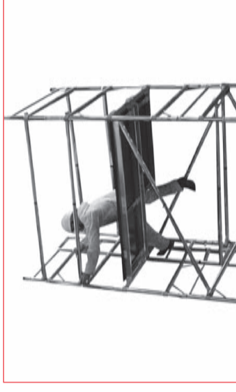
19 Dismantling is the reverse except when dismantling the handrails. Unclip the four end hooks and from the sitting position remove the handrails. Do not remove the handrails whilst standing on the platform, this would leave you at risk.
