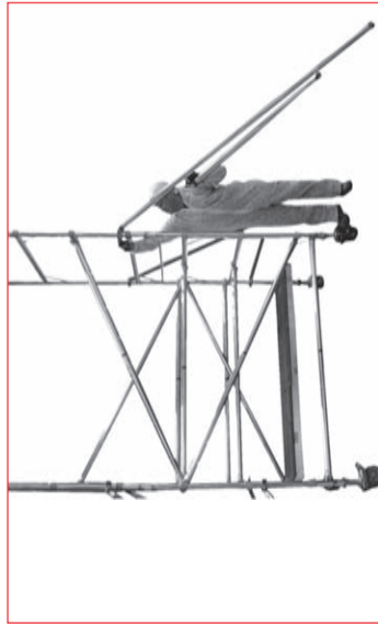
11 Secure stabilisers as soon as possible to increase tower stability. Check lower kit list to ensure the correct stabilisers are fitted.
