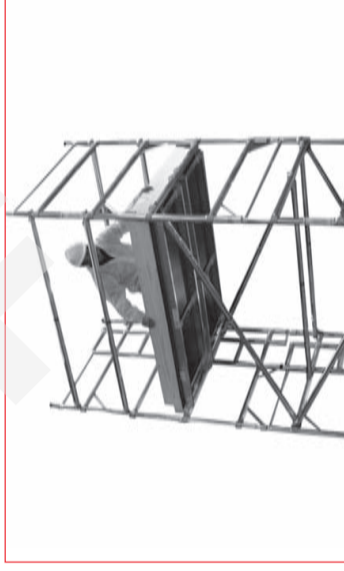
18 When handrails have been correctly fitted, fit toeboards.
